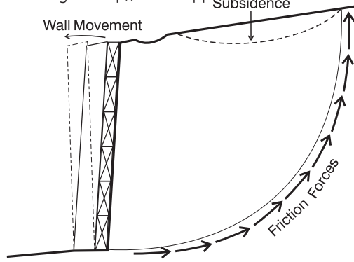
Figure 4 - Wall movement
